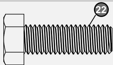
1/2-13 X 1.5 Hex Head Bolt - Zinc 1B-6486-10 (QTY. 2)
